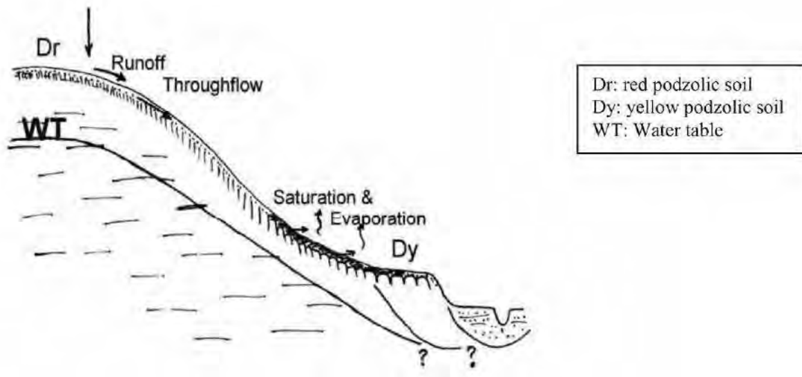
Figure 3.4: Salinity associated with shale soil landscape (Mitchell, 2000)
