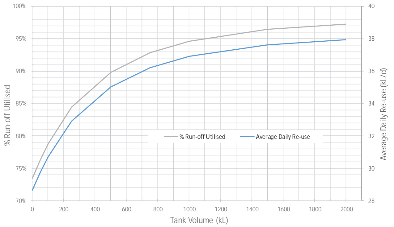
Figure 4.2: Roof water tank size vs re-use rate. (IGGC, 2015)
