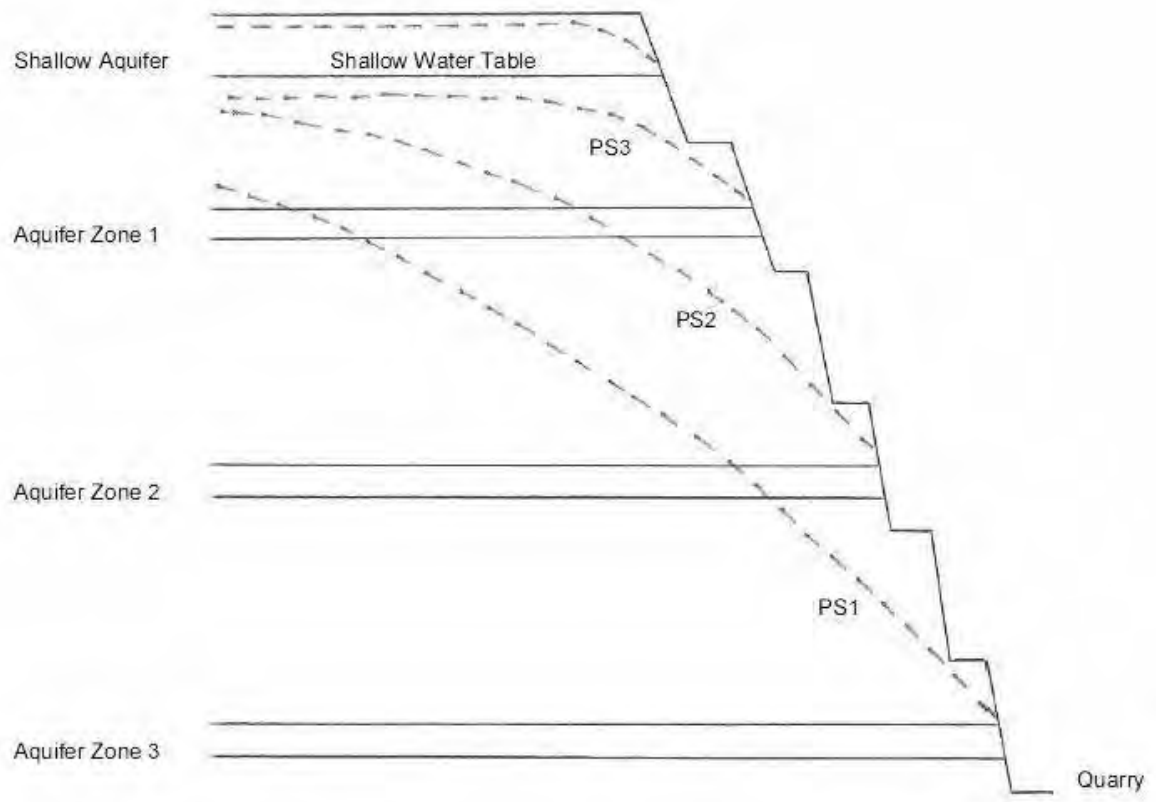
Figure 3.3: Conceptual groundwater regime (Simplified, Not to Scale). Source (IGGC (2005))
